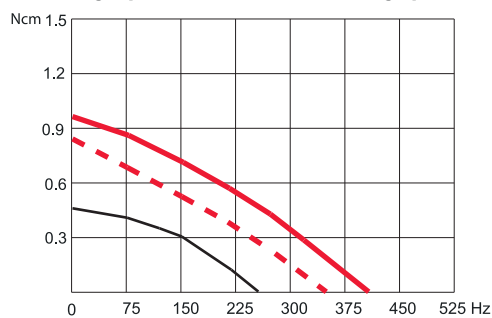
4-Phase Stepper Motor MTSU3b
