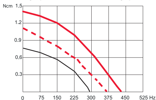
2-Phase stepper Motor MTSB3b
